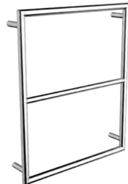
SC15 - SPACE SAVING TOWEL RACK W - 400 D - 480 P - 67 C1 - 381 C2 - 400
