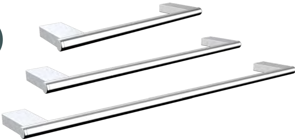
IS03/IS06/IS07/IS10 - TOWEL RAILS IS03- W - 458 D - 16 P - 80 IS06- W - 608 D - 16 P - 80 IS07- W - 358 D - 16 P - 80 IS10- W - 308 D - 16 P - 80
