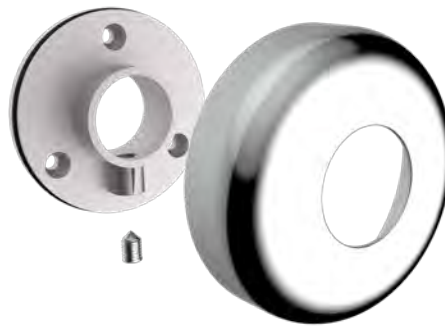
NH34 - FLANGES & COVER PLATES FOR STRAIGHT AND 'L' SHAPE RAILS (PAIR) Ø - 65 P - 20
