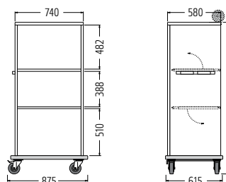
Transporting clean linen With roll-down front panel
