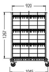
FW-16 Bottle trolley
