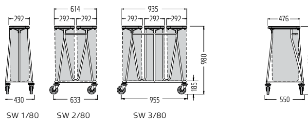
SW 2/80 Fabric bags in red and blue, alternatively with a foot pedal and locking brake
