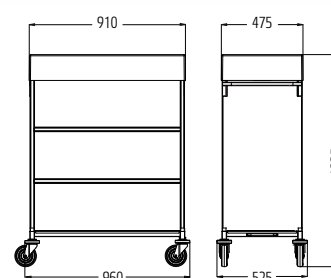
TERRACE TROLLEY PREMIUM ZP UNIQUE
